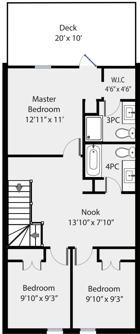
Upper Floor 800 SQFT
