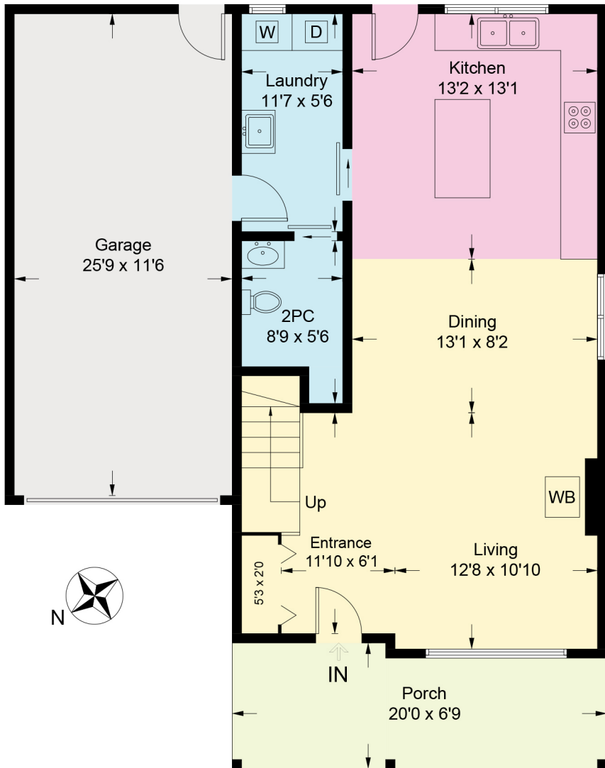
Main Floor - 692 sq ft
