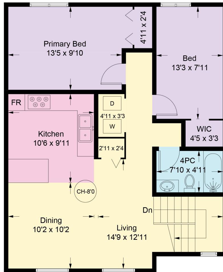
Main Floor - 828 sq ft
