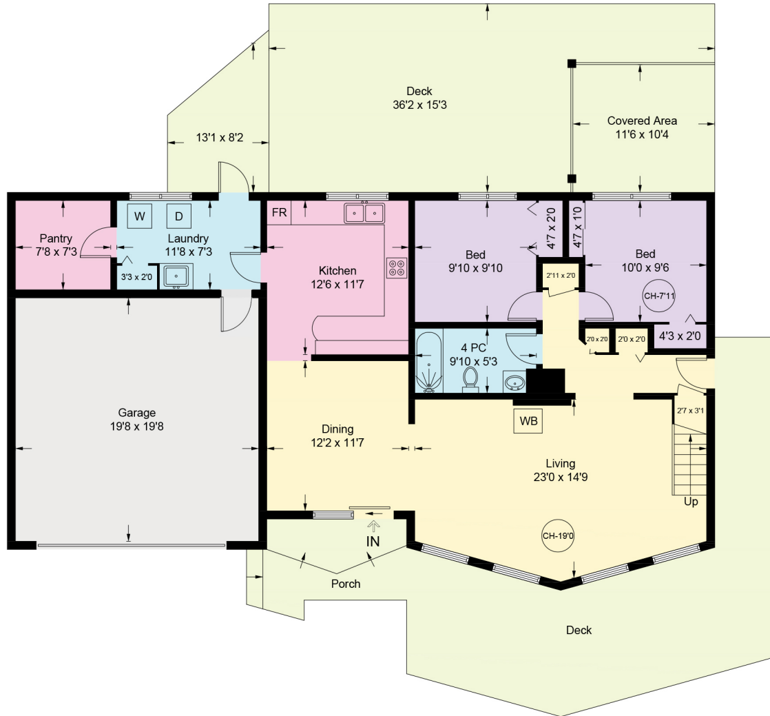
Main Floor - 1249 sq ft
