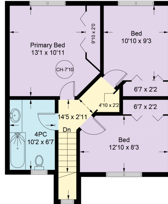
Upper Floor = 613 sq ft
